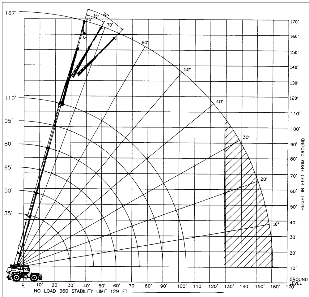
Range Diagram (33' - 110' boom)
